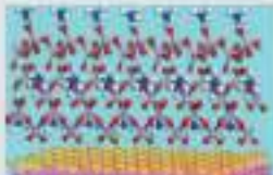
APP particles
